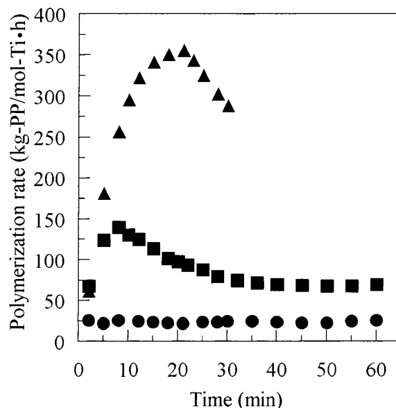
Figure 2. Rate–time profiles of propene polymerization with [ t -BuNSiMe 2 Flu]TiMe 2 using various cocatalysts: (a) B(C 6 F 5 ) 3 /Oct 3 Al (■), (b) MAO (●), (c) dried MAO (▲).
